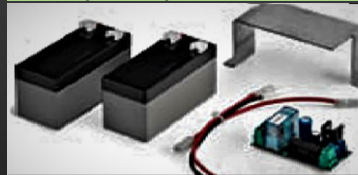
Battery Charger Kit for Heady24 control box. Comes with cby.24 v battery charger, 1.2A.h batteries and battery holder brackets.
